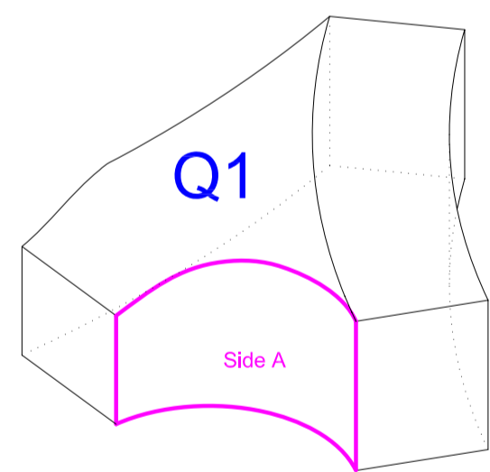
Isometric view of side A for flattened surface shown below
