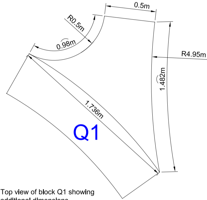
Top view of block Q1 showing additional dimensions
