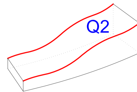
Isometric view showing edges in red colour to be rounded at 30mm radius
