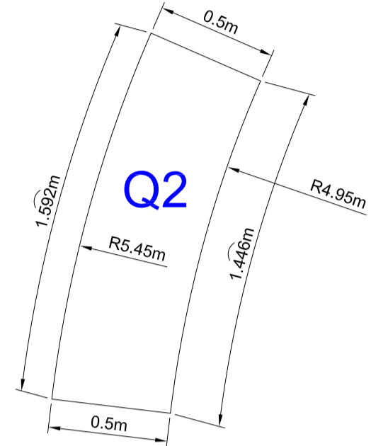
Top view of block Q2 showing dimensions
