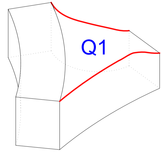
Isometric view showing edges in red colour to be rounded at 30mm radius
