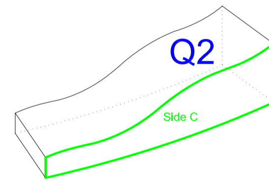
Isometric view of side C for flattened surface shown below
