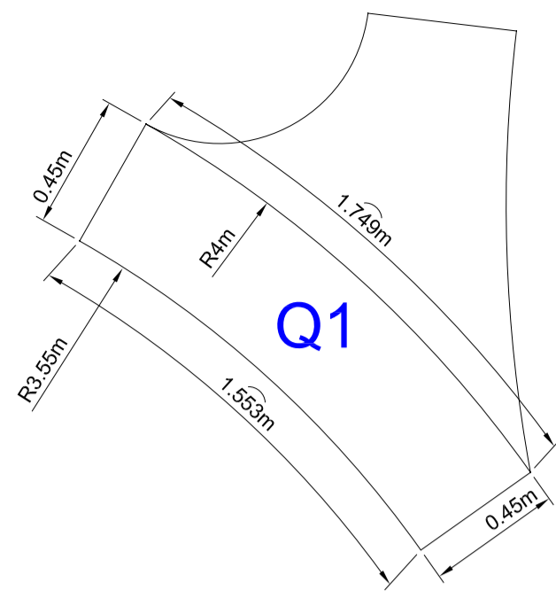
Top view of block Q1 showing dimensions
