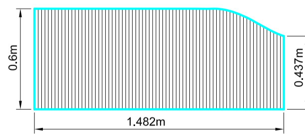
Flattened surface of side B
