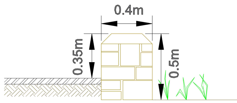
Wall - Typical Section
